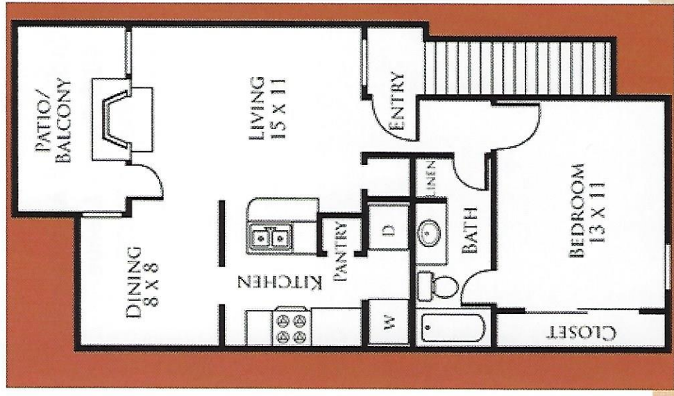
One Bedroom 700 Sq Ft
